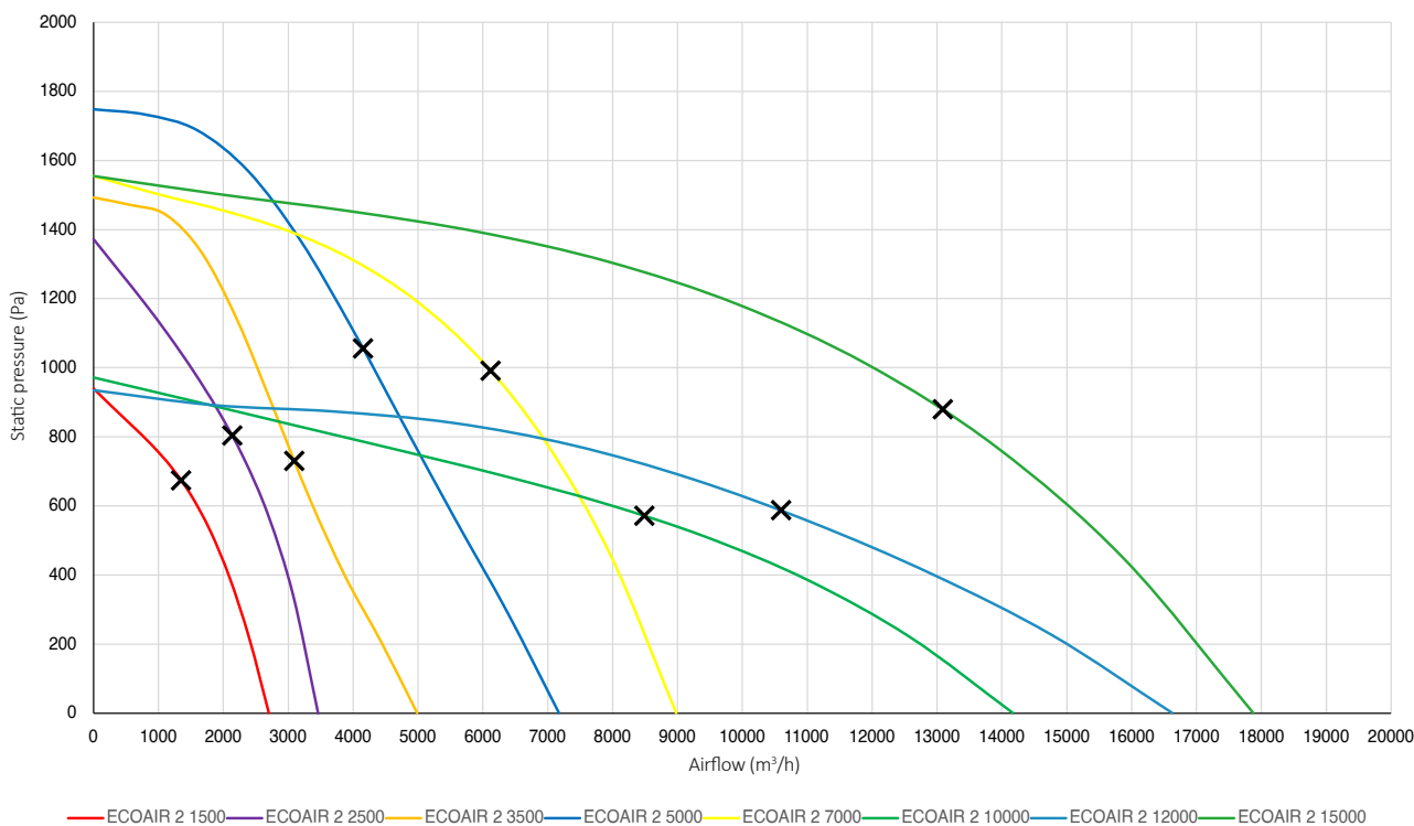
ECOAIR 2 ePM1 50%/F7 + WATER COIL
