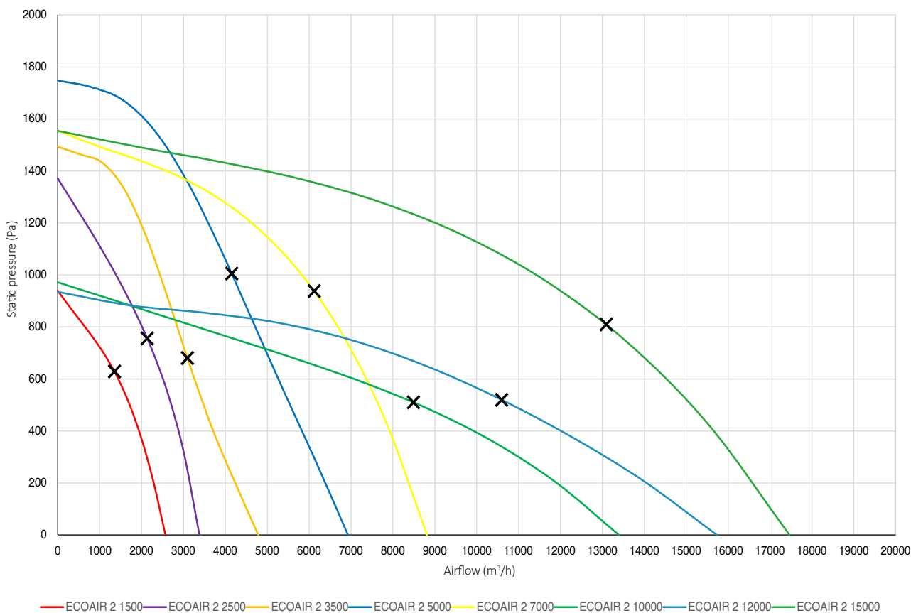
ECOAIR 2 ePM10 50%/M5 + ePM1 50%/F7 + WATER COIL
