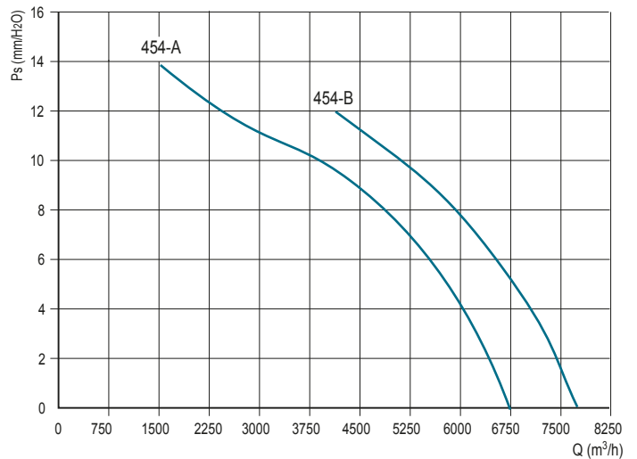
DUCT-M 450
