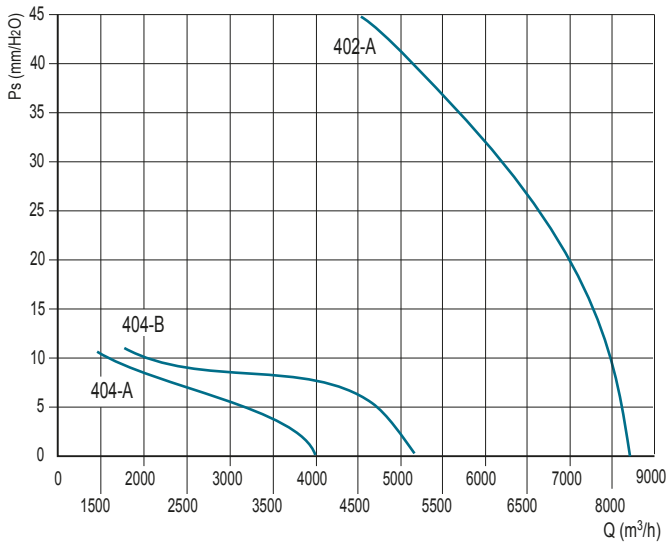
DUCT-M 400
